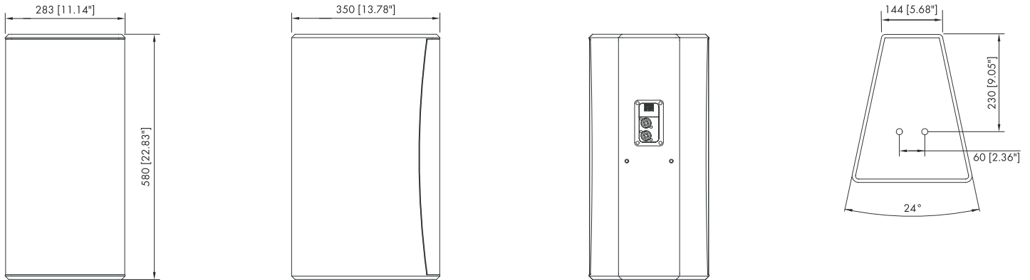
10S cabinet dimensions in mm [inch]
